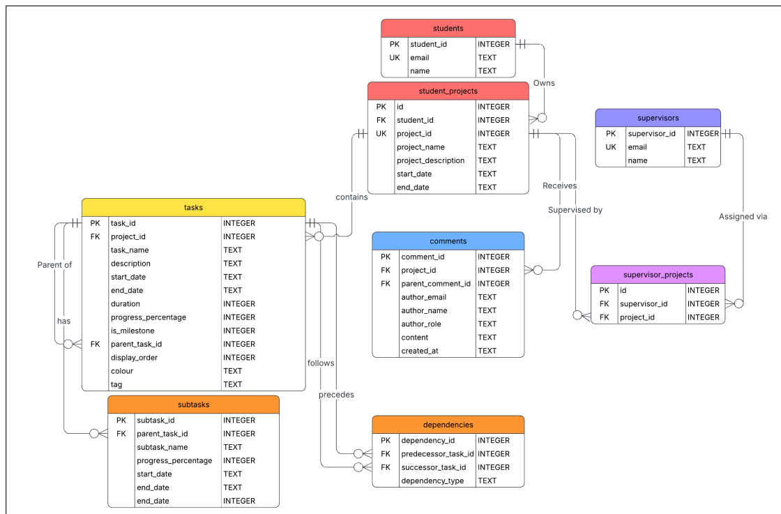
Fig. 1. Entity-Relationship Diagram.
